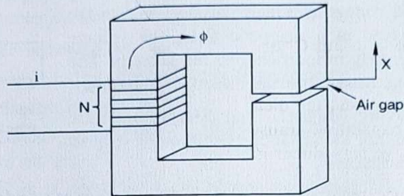
Fig. 2.13. Electromagnetic Transducer.
