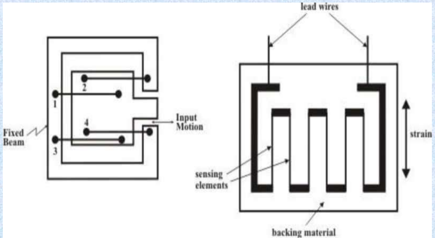
Fig. 6 (a) Unbonded metallic strain gauge, (b) bonded metal foil type strain gauge
