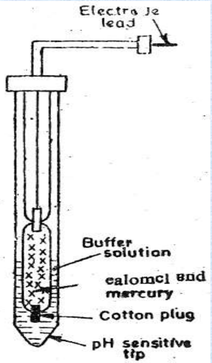
(b) Measuring electrode.
