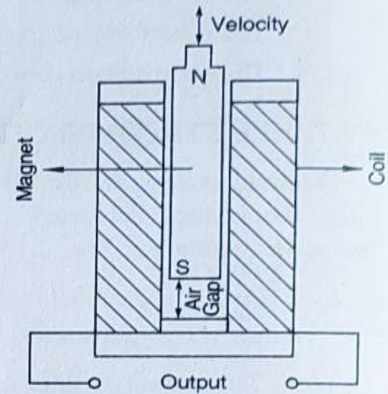
Fig. 2.14. Moving magnet type electromagnetic transducer.
