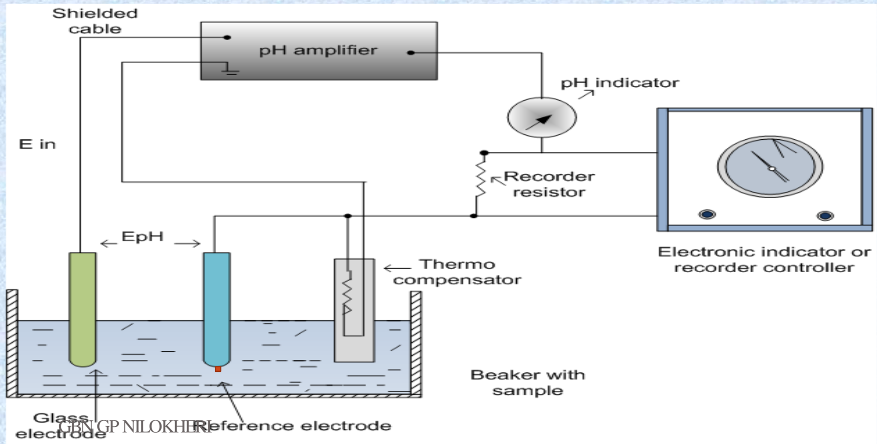
Circuit for electronic pH measurement
