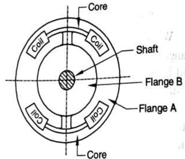
(b) Arrangement using four Inductive Transducers
